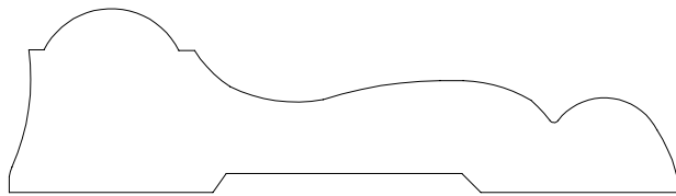
CHAIRRAIL 53133 7/8" X 3 3/16"
