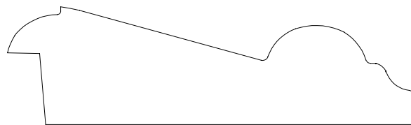
CHAIRRAIL 5306 7/8" X 3 1/32"
