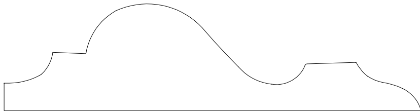
CHAIRRAIL 54253 1 3/32" X 4 9/32"
