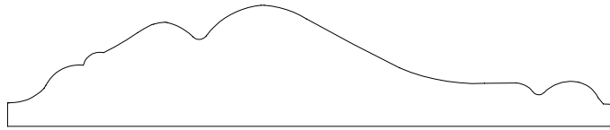
CHAIRRAIL 535014 23/32" X 3 17/32"
