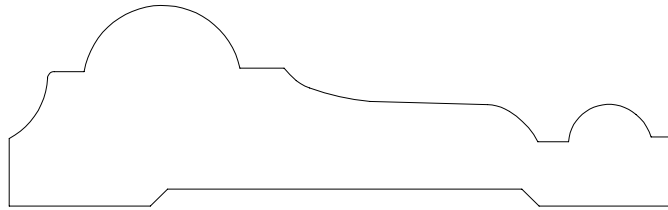
CHAIRRAIL 535016 1 1/16" X 3 1/2"
