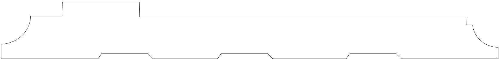
CHAIRRAIL 9869 1" X 8 11/16"
