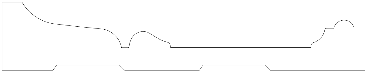
CHAIRRAIL 5625 1 3/16" X 6 1/4"
