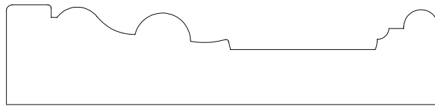
CHAIRRAIL 53254 3/4" x 3 1/4"
