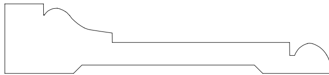
CHAIRRAIL 535017 3/4" X 3 1/2"
